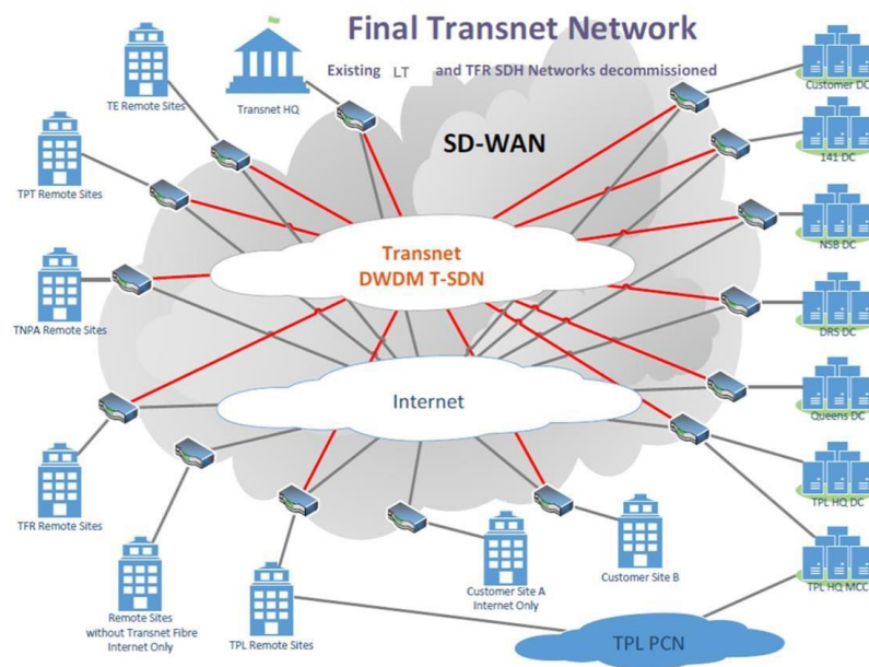
Figure 2: The high level envisaged TO-BE state of the Transnet network
